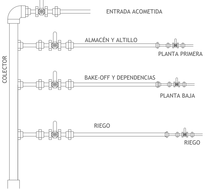
DETALLE COLECTOR AGUA POTABLE
