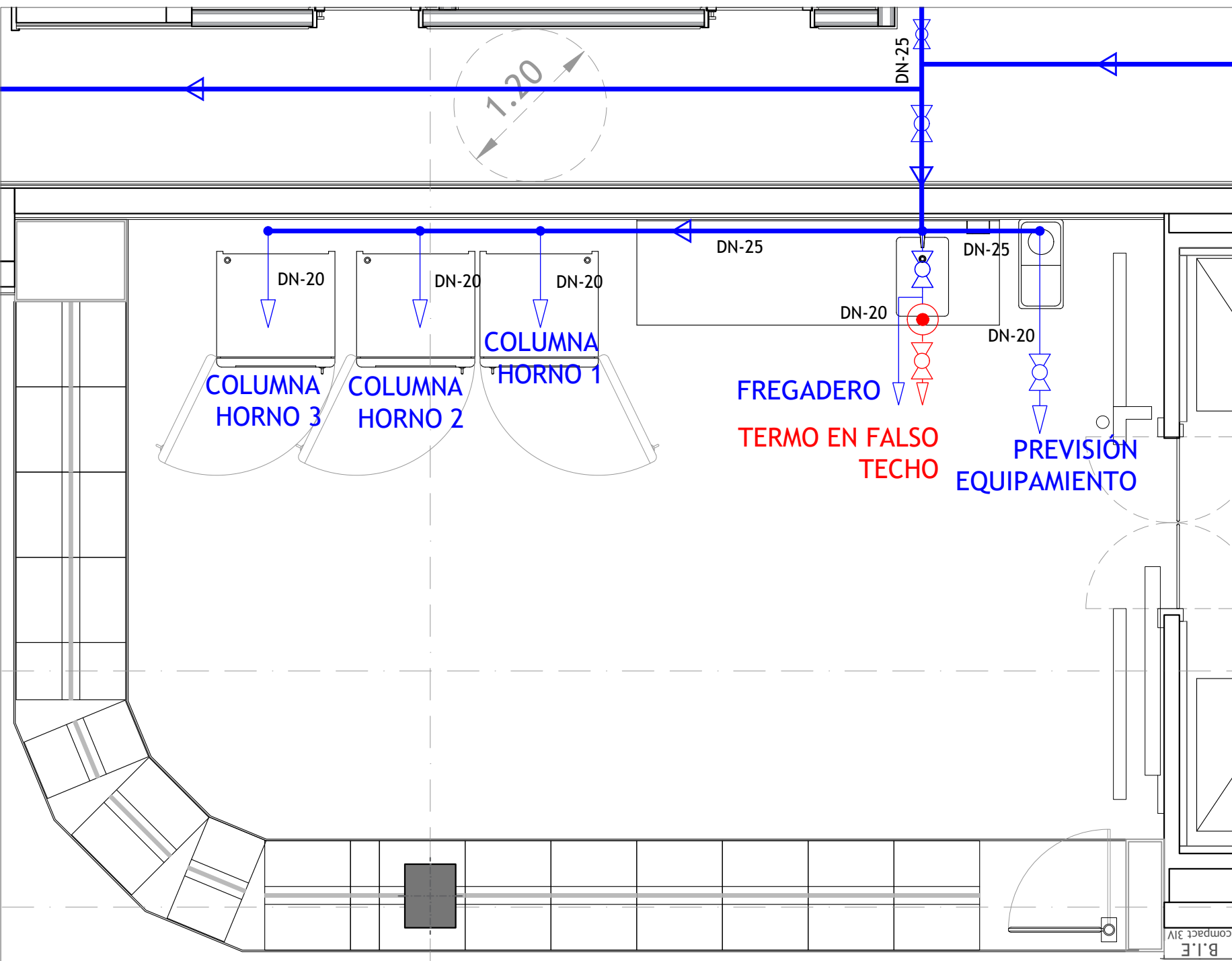
BAKE OFF_E 1/40
