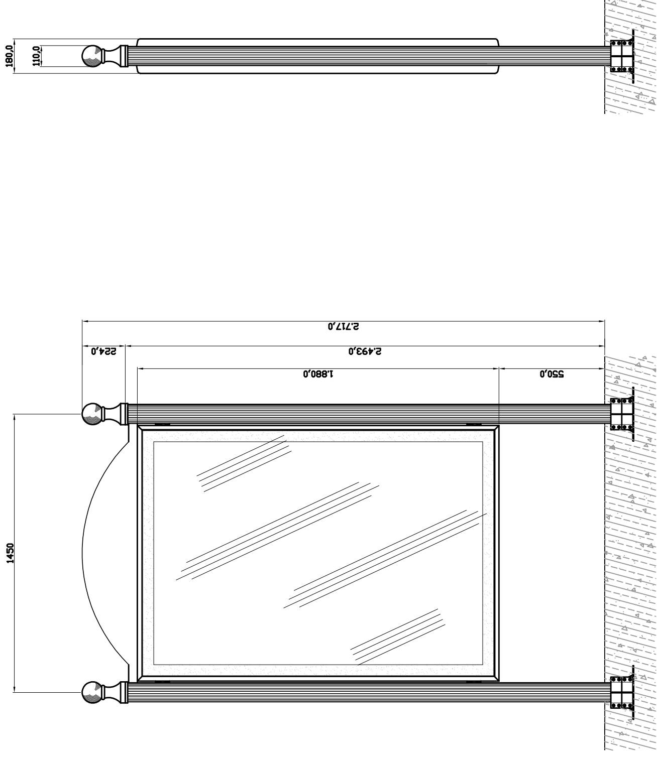
VISTA FRONTAL
