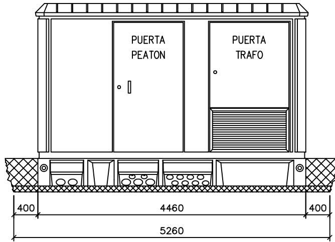
VISTA FRONTAL
